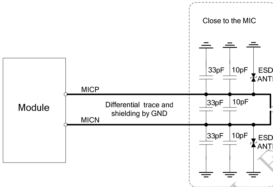
Figure 31: Microphone reference circuit
