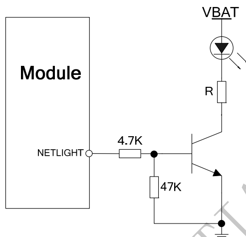
Figure 45: Reference circuit of NETLIGHT
