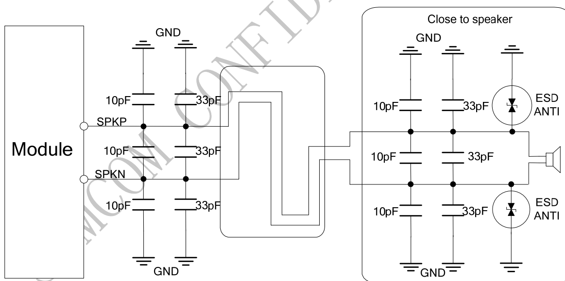
Figure 30: Speaker reference circuit
