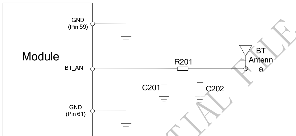
Figure 50: Bluetooth antenna matching circuit
