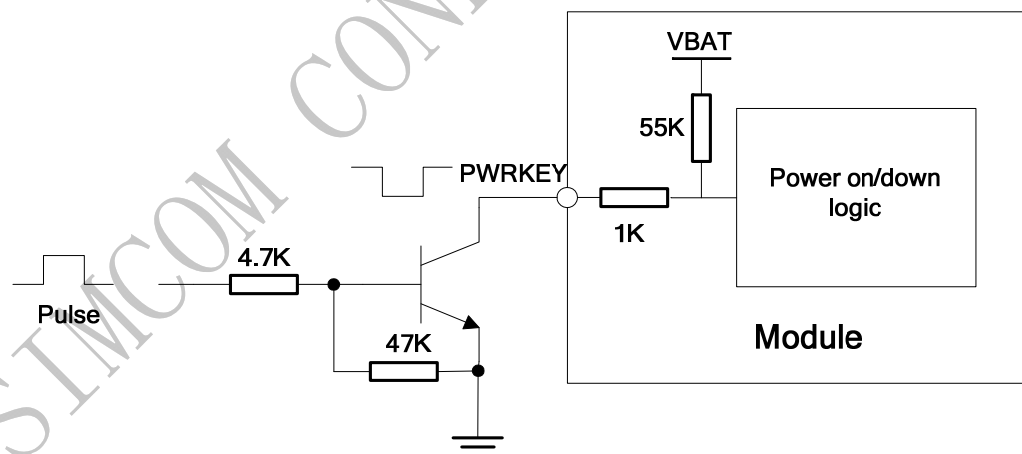
Figure 10: Power on/down module using transistor
