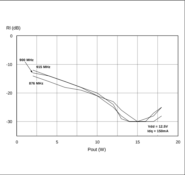
Figure 25. Input Return Loss vs Output Power
