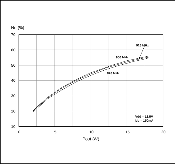
Figure 24. Drain efficiency vs. output power
