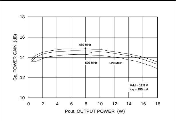
Figure 6. Power gain vs output power
