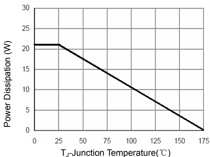
Figure 9 Figure 9 Power De-rating
