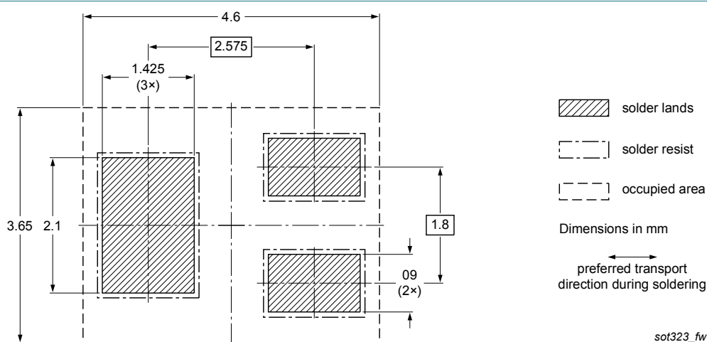
Figure 18. Wave soldering footprint for SOT323 (SC-70)
