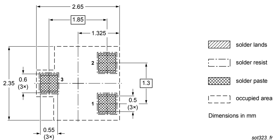
Figure 17. Reflow soldering footprint for SOT323 (SC70)
