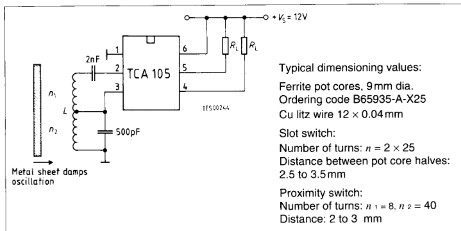
Circuit Diagram
