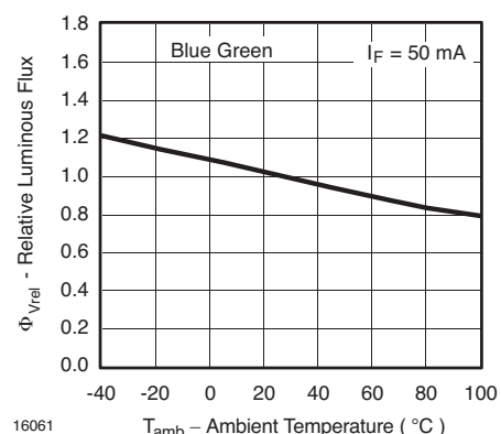
Figure 30. Rel. Luminous Flux vs. Ambient Temperature
