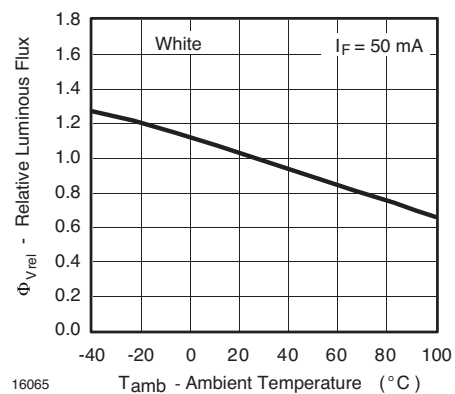
Figure 42. Rel. Luminous Flux vs. Ambient Temperature
