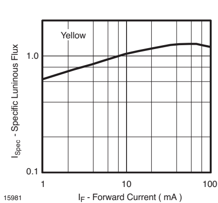
Figure 19. Specific Luminous Flux vs. Forward Current
