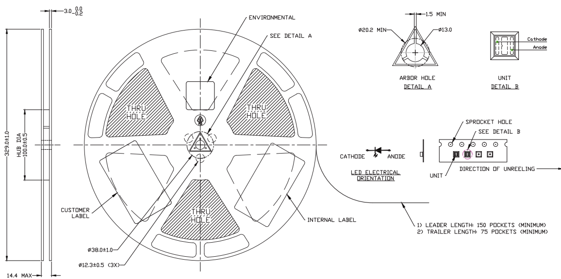
Figure 10a. Reel dimensions for LUXEON SunPlus 20 Line
