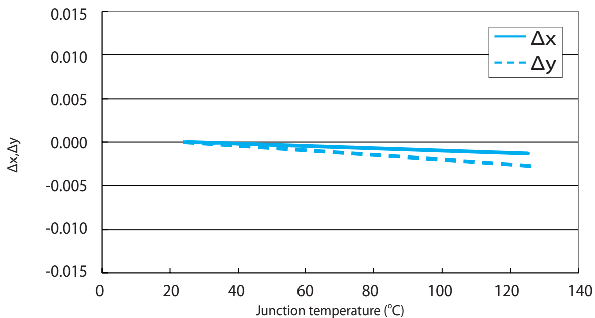
\Delta x, \Delta y vs. Junction temperature for Edixeon S White
