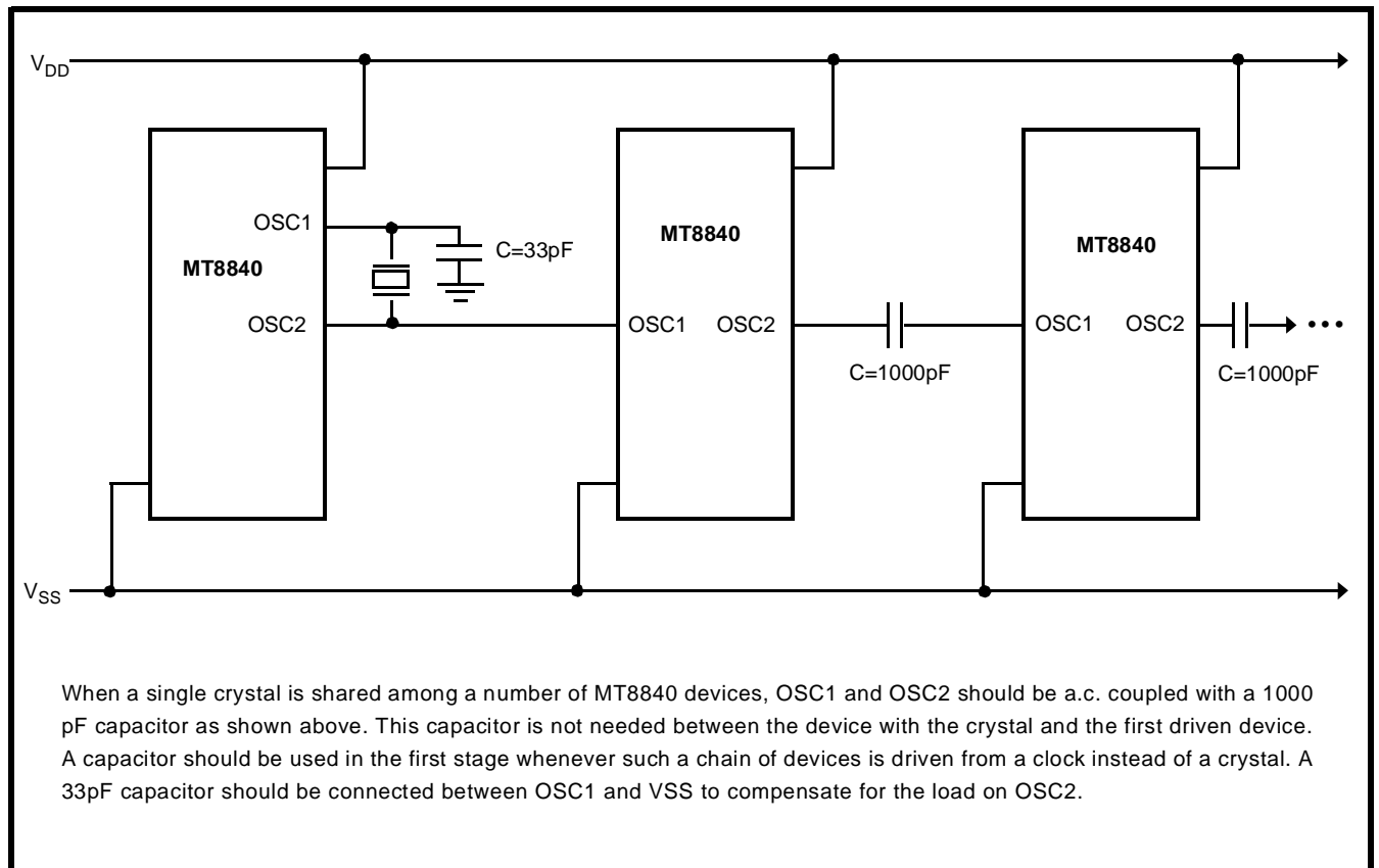
Figure 6 - Crystal Oscillator Connections for Driving Multiple MT8840s
