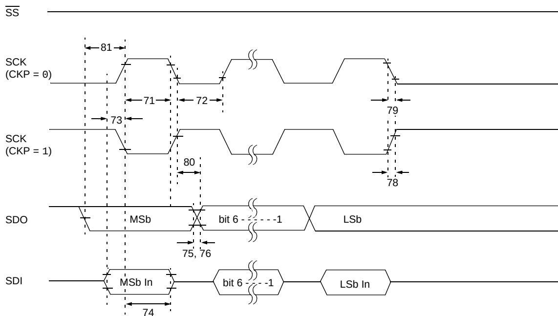
FIGURE 17-13: SPI MASTER MODE TIMING (CKE = 1, SMP = 1)
