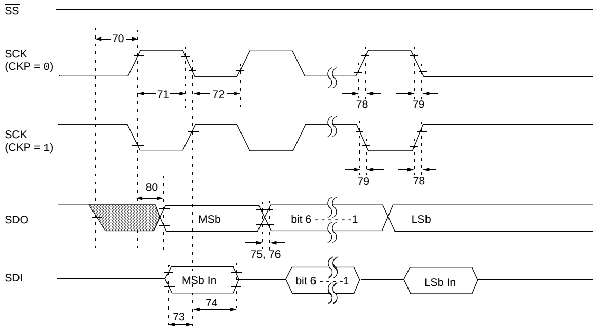
FIGURE 17-12: SPI MASTER MODE TIMING (CKE = 0, SMP = 0)
