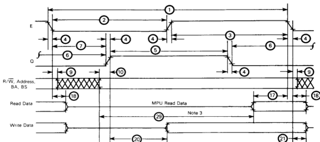
FIGURE 1 — BUS TIMING
