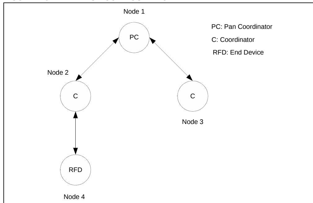
FIGURE 4-6: MESH CONFIGURATION
