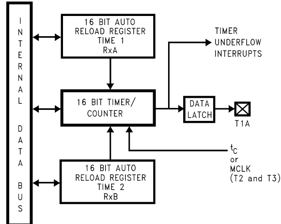
Figure 5-10. Timer in PWM Mode
