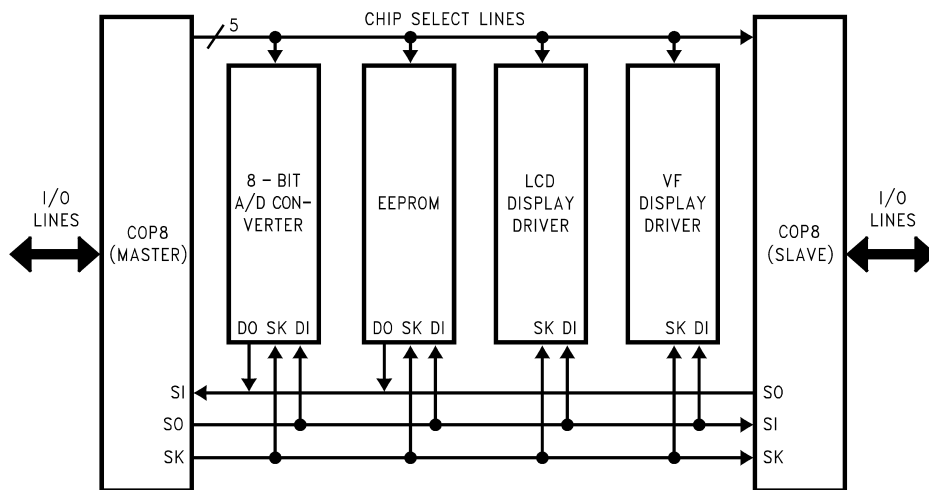
Figure 5-23. MICROWIRE/PLUS Application
