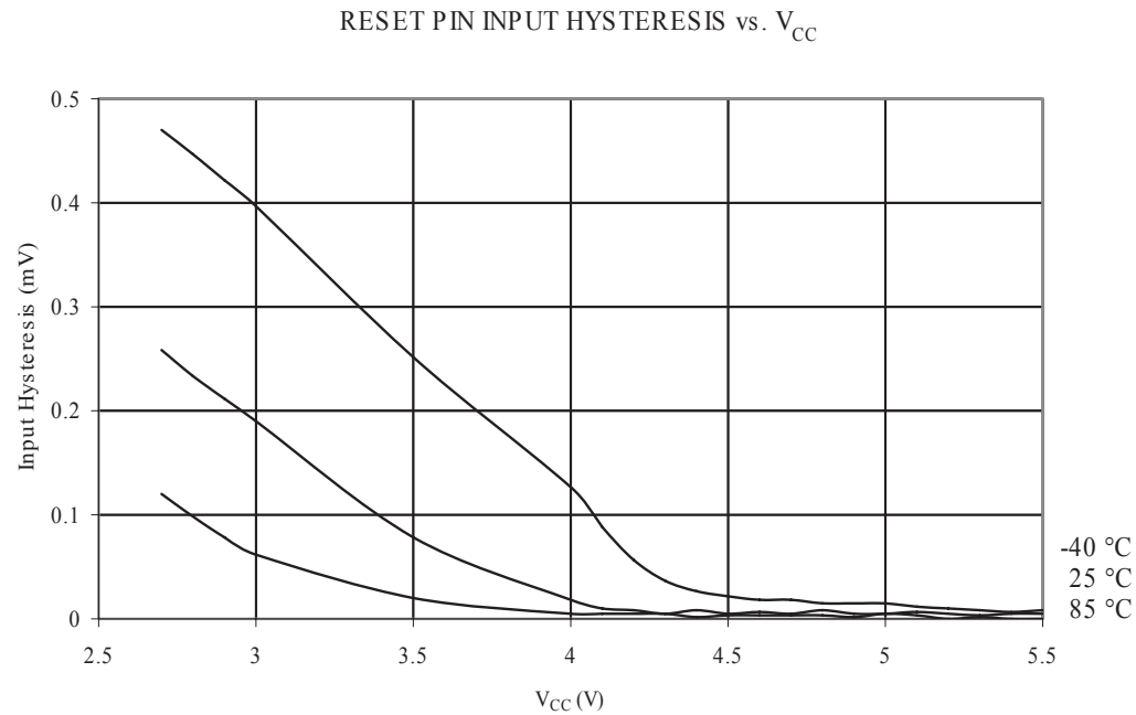
Figure 33-56 Reset Input Pin Hysteresis vs. V_{CC}
