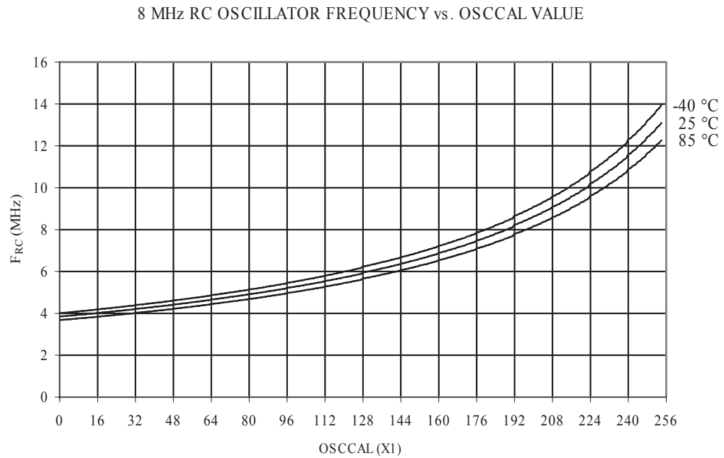
Figure 33-44 8MHz RC Oscillator Frequency vs. Oscal Value
