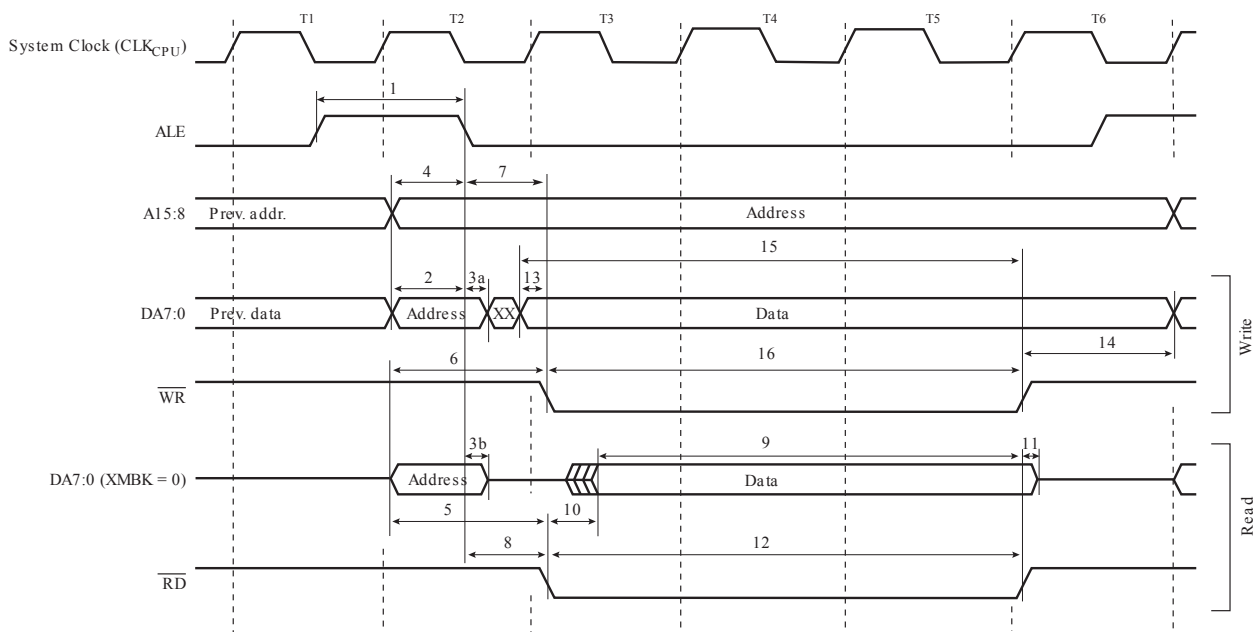
Figure 32-11 External Memory Timing (SRWn1 = 1, SRWn0 = 1)
