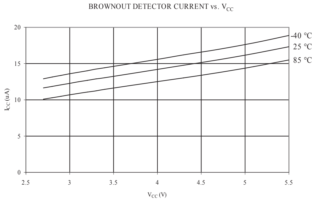
Figure 33-45 Brownout Detector Current vs. V_{CC}
