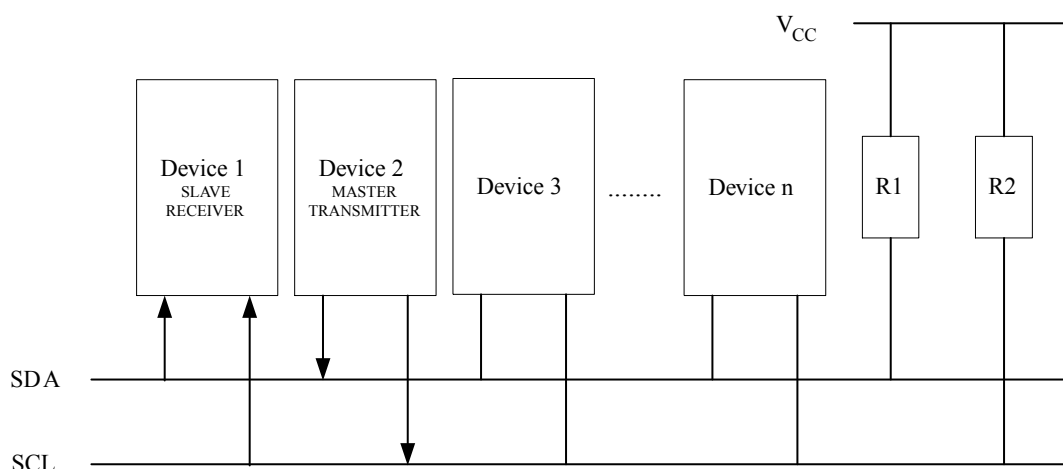
Figure 26-15 Data transfer in Slave Receiver mode
