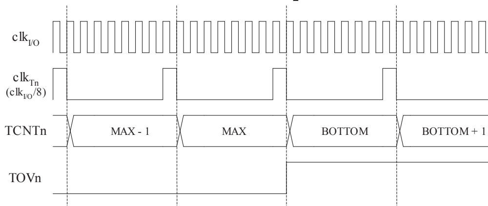
Figure 22-9 Timer/Counter Timing Diagram, with Prescaler ( f_{\text{clk}_{I/O}}/8 )
