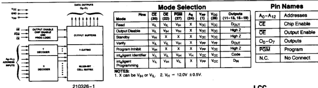
Figure 1. Block Diagram
