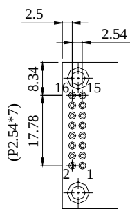
PIN DETAIL
