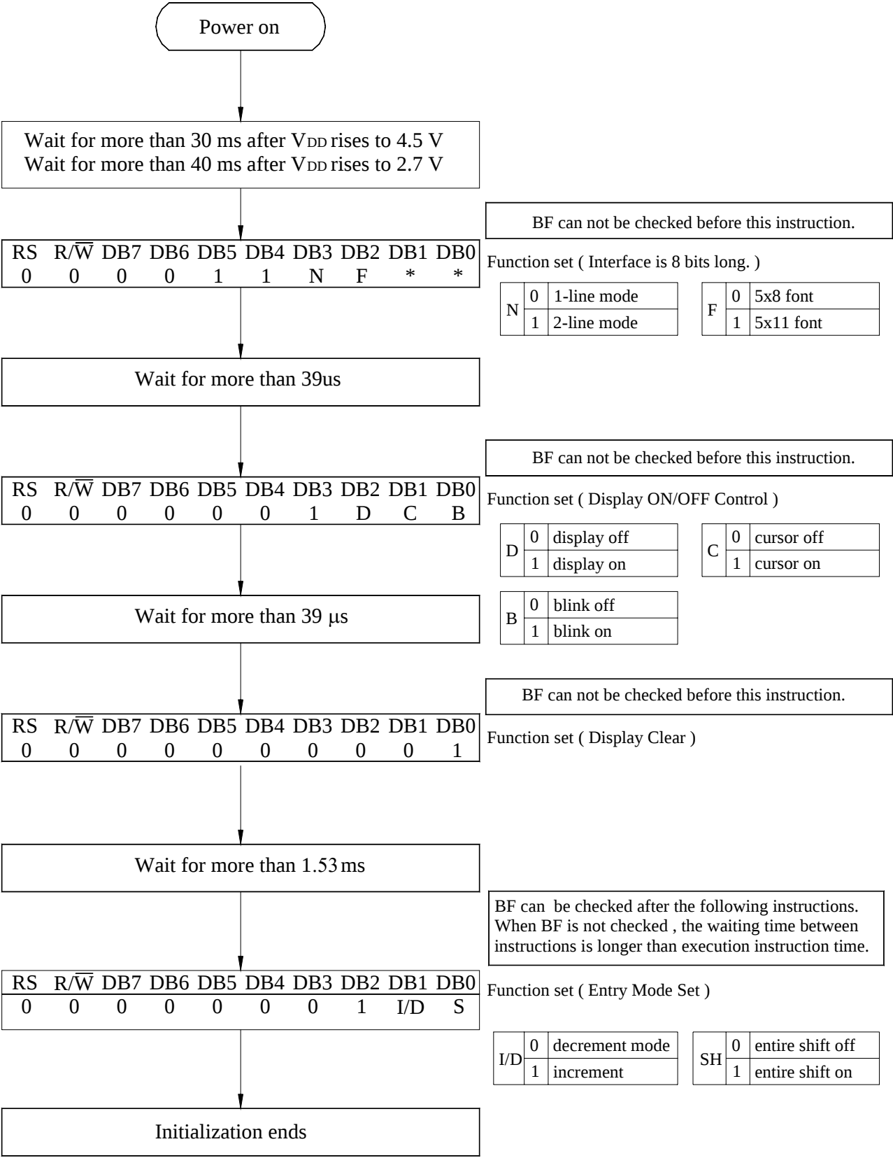
8-Bit Ineterface
