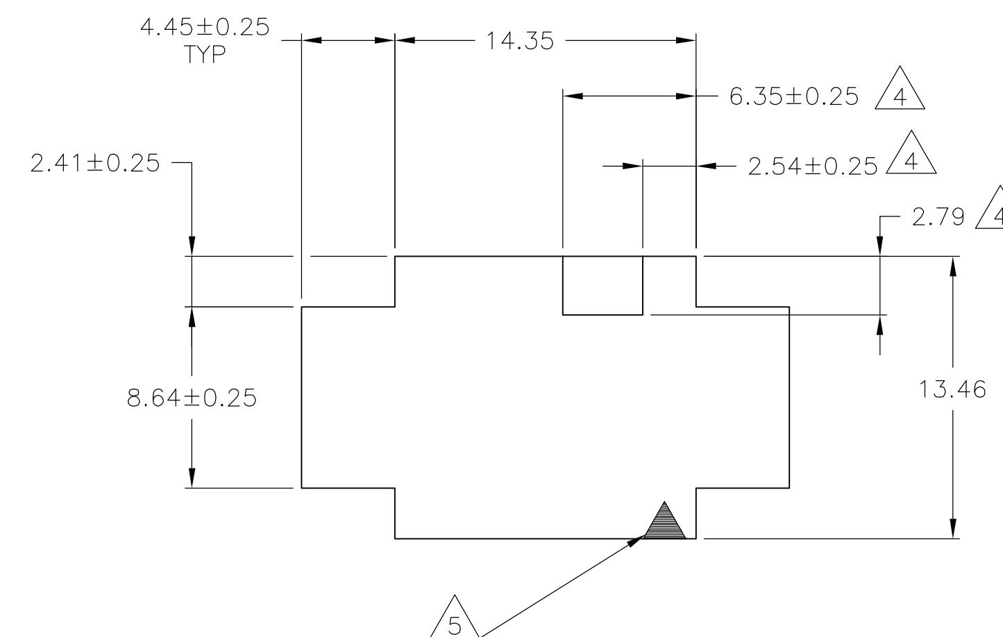
RECOMMENDED PANEL CUTOUT
