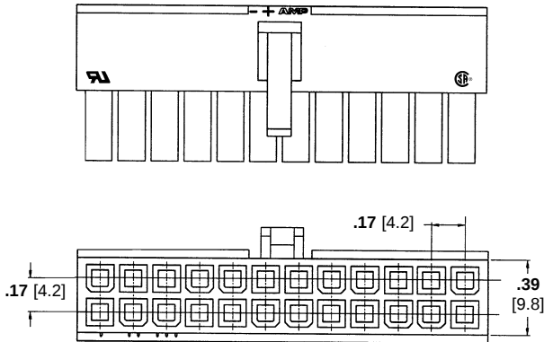
Receptacle Housing
