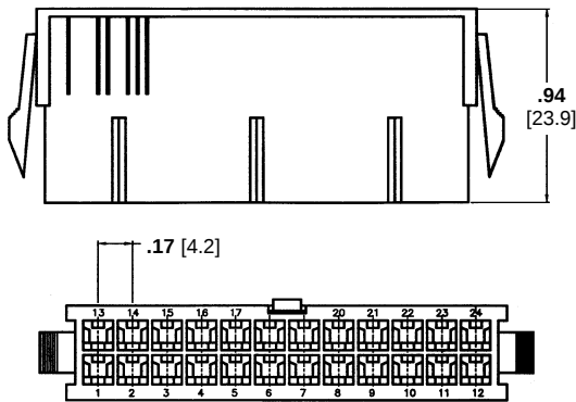
Panel Mount Plug Housing
