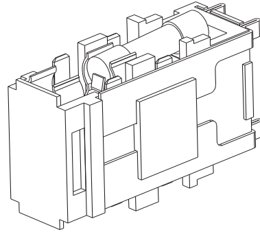
Fuseholder shown with 5x20mm fuse
