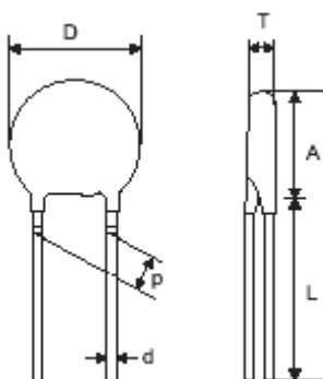
S type (straight lead)
