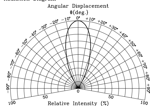
Radiation Diagram
