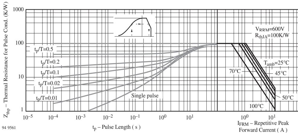
Figure 7. Thermal Response
