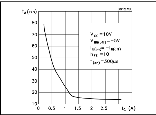
Figure 12. Switching times resistive load
