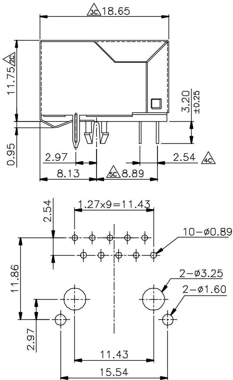
PCB LAYOUT/TOP VIEW
