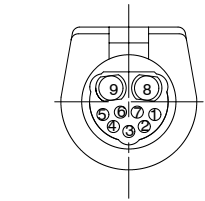
Receptacle Viewed from the Mating Side
