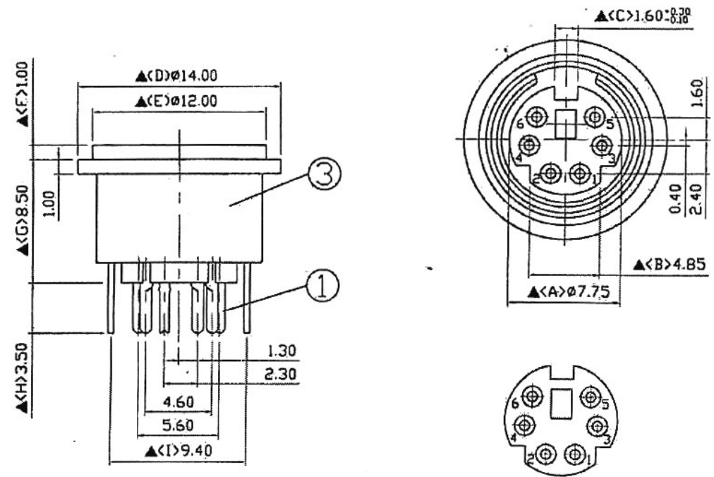
Arrangement of Contact
