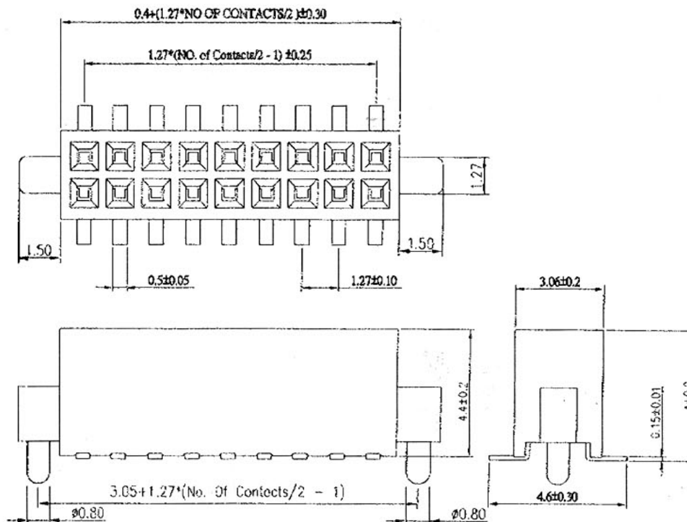
Pin Chart
