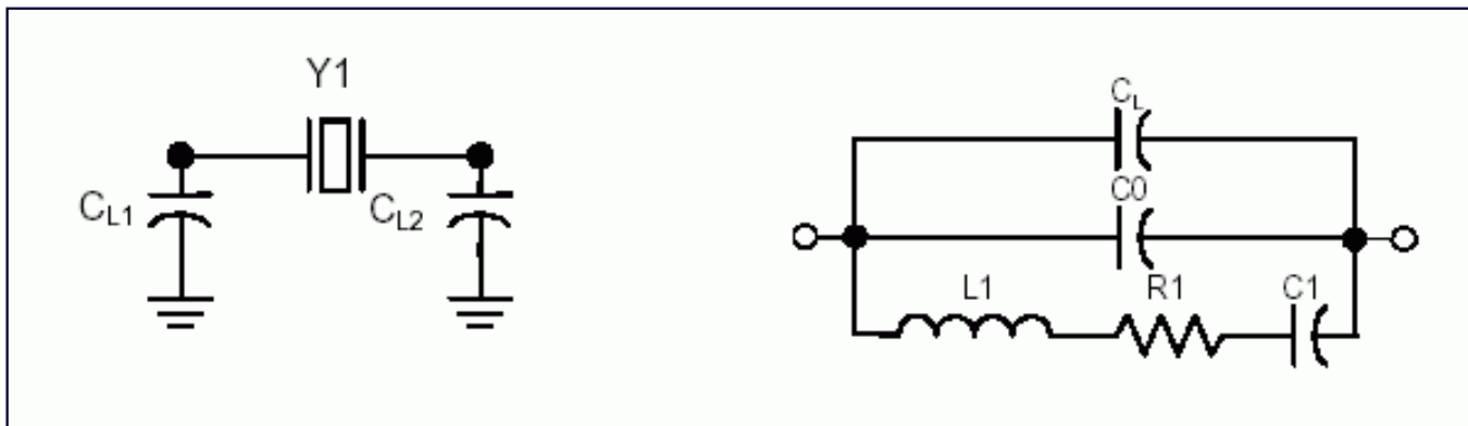
Figure 4. Crystal Load Capacitors and Equivalent Parallel Load
