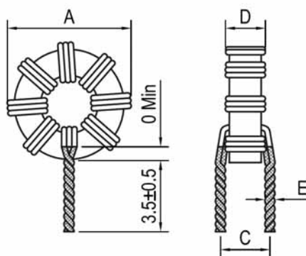
Figure 2 (multiwire type)
