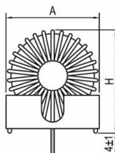
Figure:2 (TBKM type, Use KM series base)
