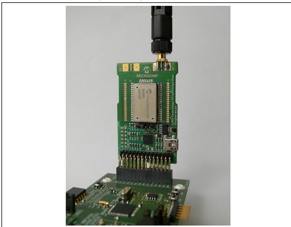
FIGURE 1-3: RN2903 LoRa™ TECHNOLOGY PICtail™/PICtail PLUS DAUGHTER BOARD CONNECTED TO PIC18 WIRELESS DEVELOPMENT BOARD
