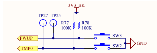
Figure 3-32. Tamper 0 & Force Wake-up Buttons
