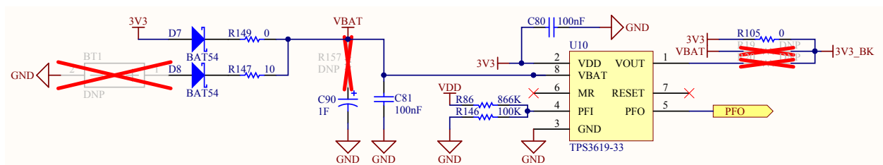
Figure 3-19. Back-up Circuit
