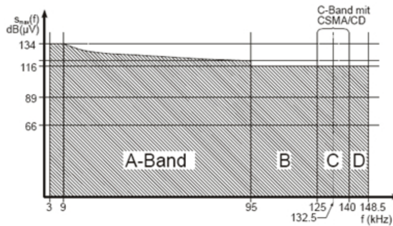
Figure 4-1. CENELEC Bands
