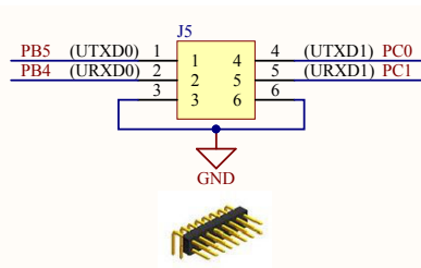
Figure 3-36. Debug UARTs over 3.3 Volts Levels
