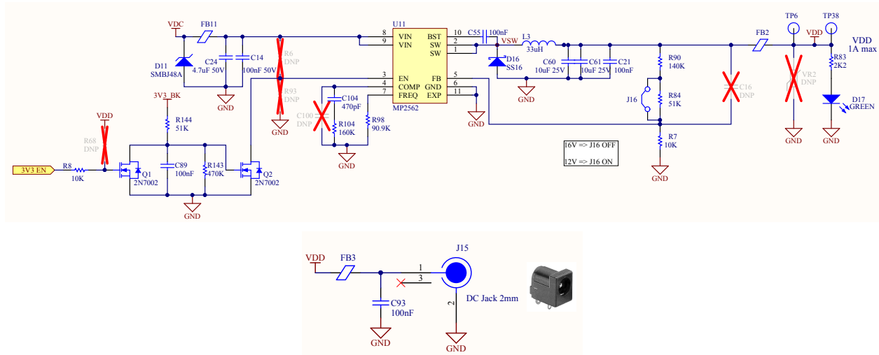
Figure 3-16. V_{DD} Buck Converter Design
