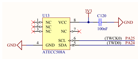
Figure 3-27. CryptoAuthentication Schematic
