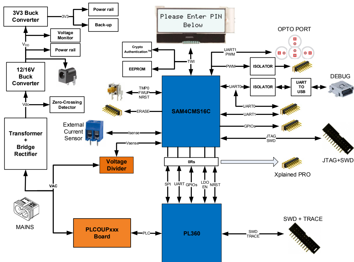
Figure 3-2. PL360MB Board Architecture
