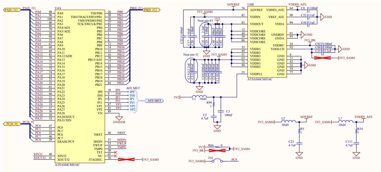
Figure 3-5. SAM4CMS Microcontroller
