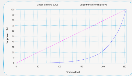
DALI-2 Dimming Curve
