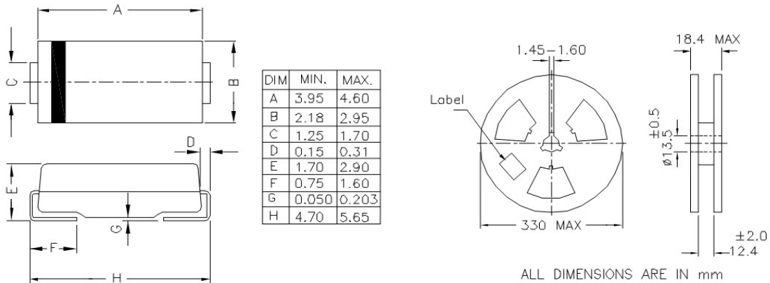
D0-214AC (SMA) Package & Reel Taping Specification
