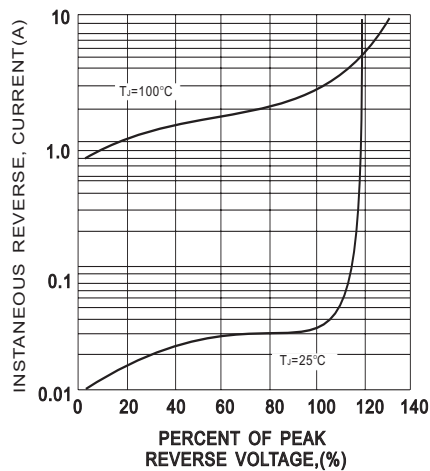
FIG. 3-TYPICAL REVERSE CHARACTERISTICS
