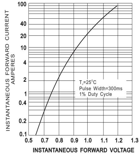
FIG. 2-TYPICAL INSTANTANEOUS FORWARD CHARACTERISTICS PER ELEMENT
