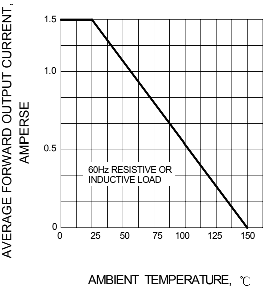
FIG.2 – FORWARD DERATING CURVE
