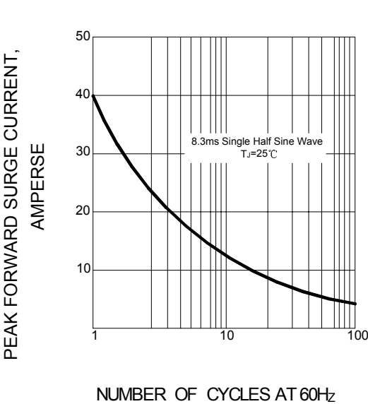
FIG.1 – PEAK FORWARD SURGE CURRENT
