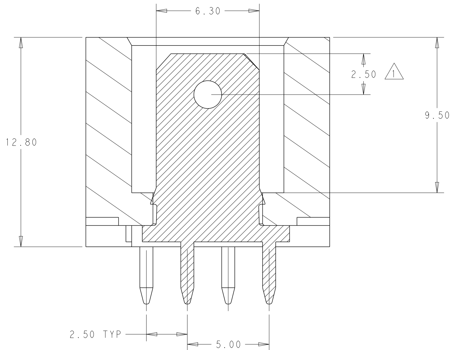
SECTION F - F
