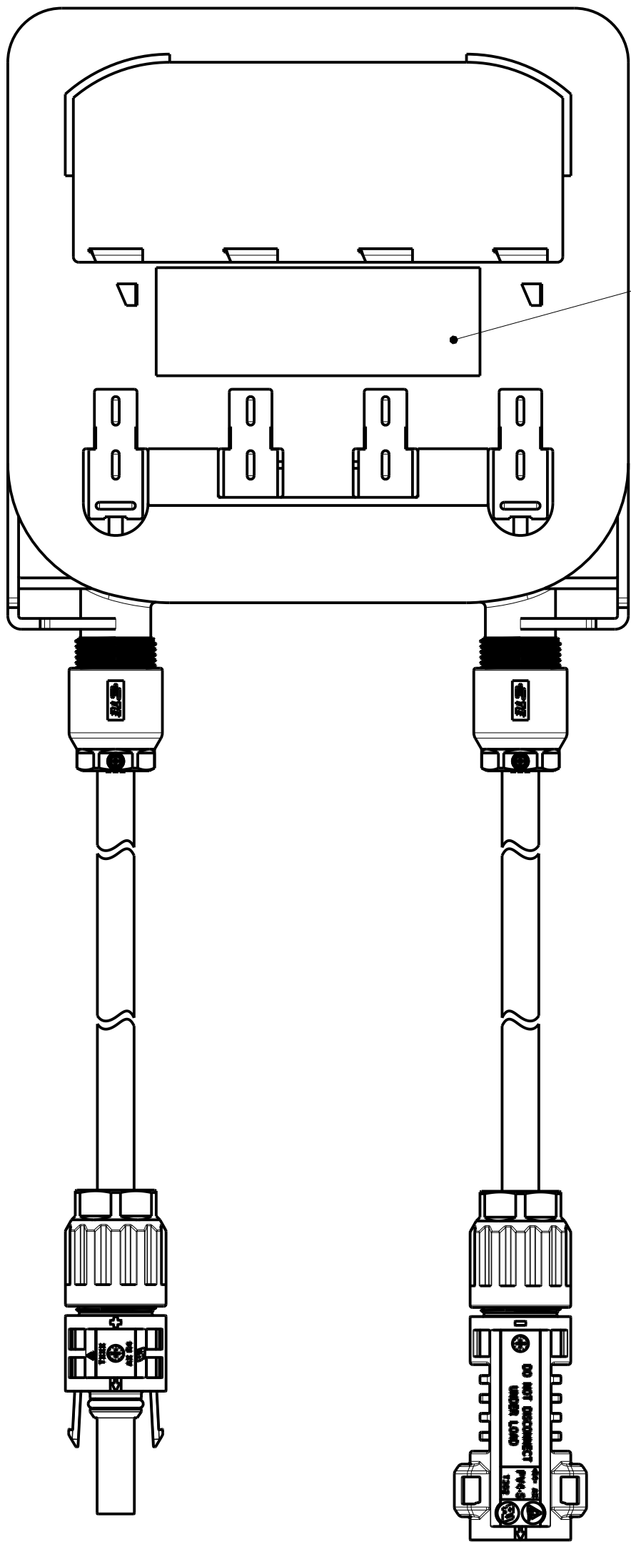
REAR VIEW OF 1, 2 & 3 AS SHOWN WITH MOUNTING TAPE
