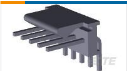
TE Part #640457-5 05P MTA100 HDR ASSY SQ R/A F/L
