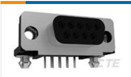
TE Part #5747844-4 09 MSFL RCPT RA 318 (IN, FM,BL)
