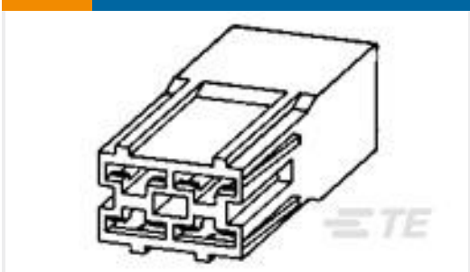
TE Model / Part #280073 FF 375 REC HSG 4P NYLON NAT
