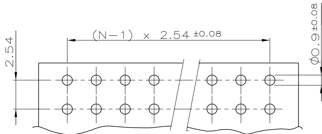
P.C.-BOARD HOLE-PATTERN
