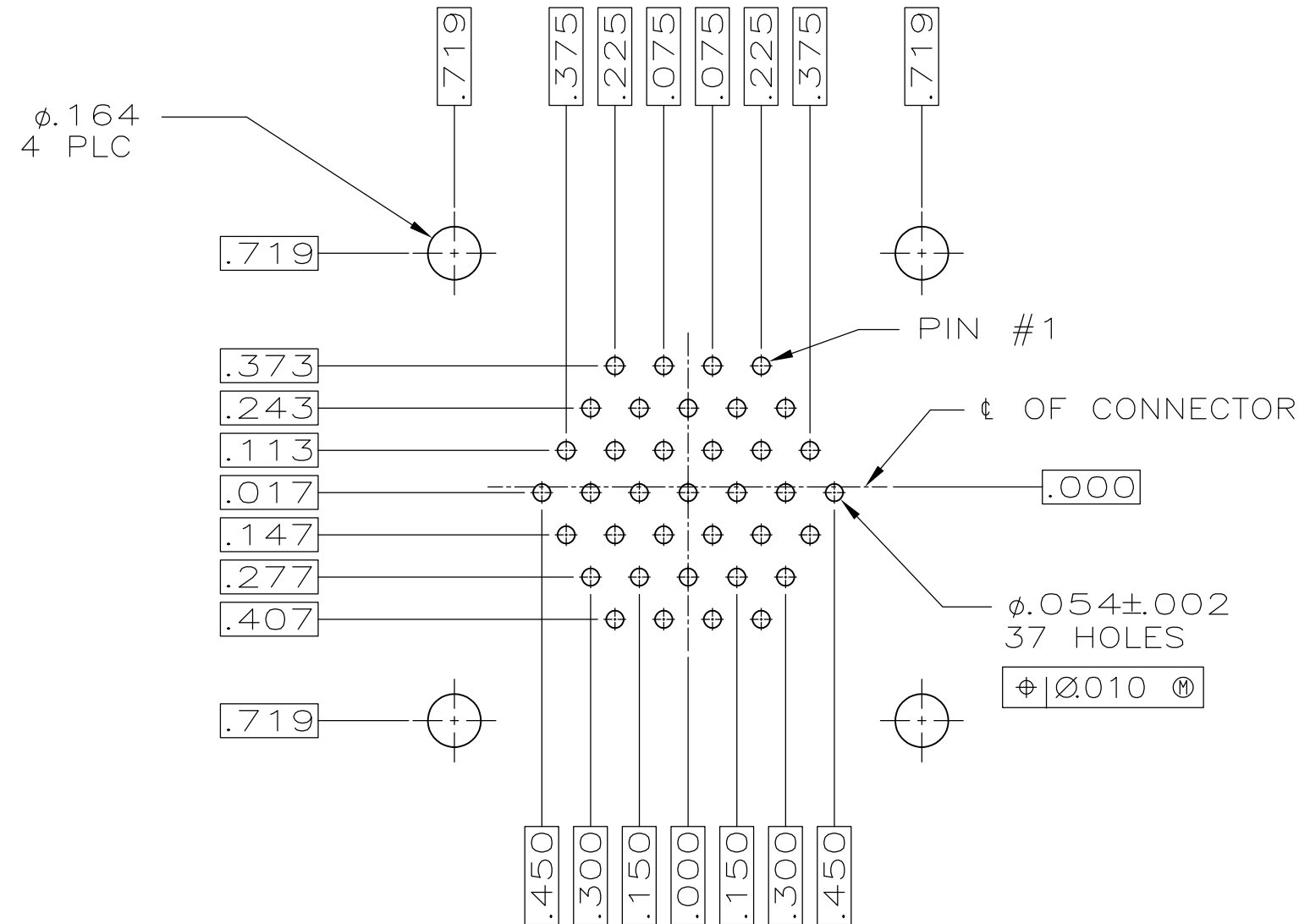
RECOMMENDED P.C. BOARD LAYOUT
