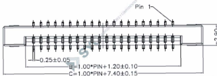
Contact Dimension
