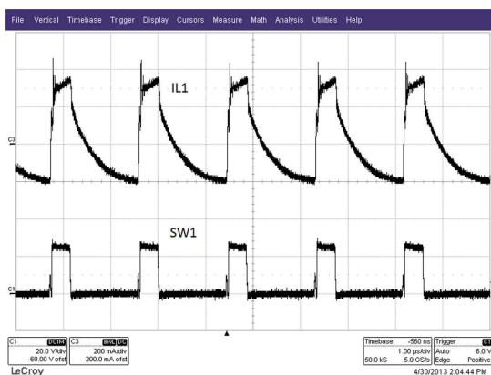
Figure 8-9. Steady State Waveform ( V_{IN} = 48\text{ V} , I_{OUT1} = 100\text{ mA} , I_{OUT2} = 200\text{ mA} )
