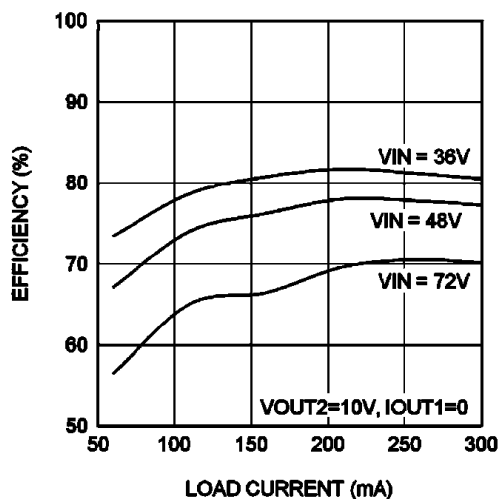
Figure 8-11. Efficiency at 750 kHz, V_{OUT1} = 10\text{ V}
