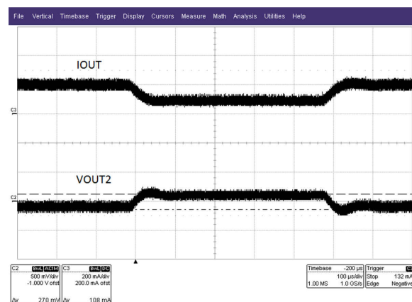
Figure 8-10. Step Load Response ( V_{IN} = 48\text{ V} , I_{OUT1} = 0\text{ A} , Step Load on I_{OUT2} = 100\text{ mA} to 200\text{ mA} )
