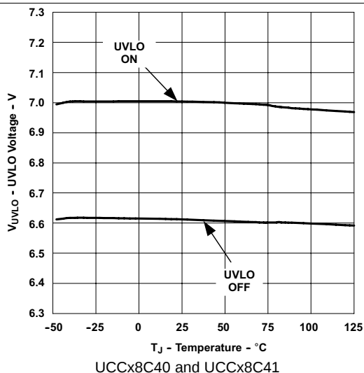
Figure 11. Undervoltage Lockout vs Temperature
