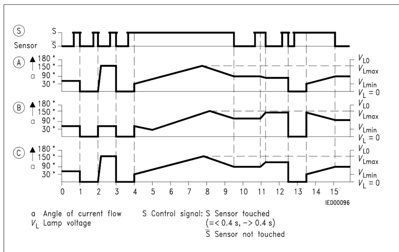
Figure 3 Control Behaviour of the 3 Operating Modes
