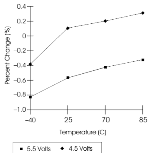
Graph 2-44: Oscillator Stability
