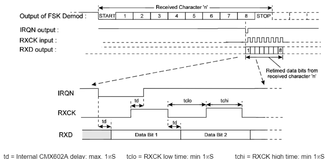
Figure 5a : FSK Operation With Data Retiming
