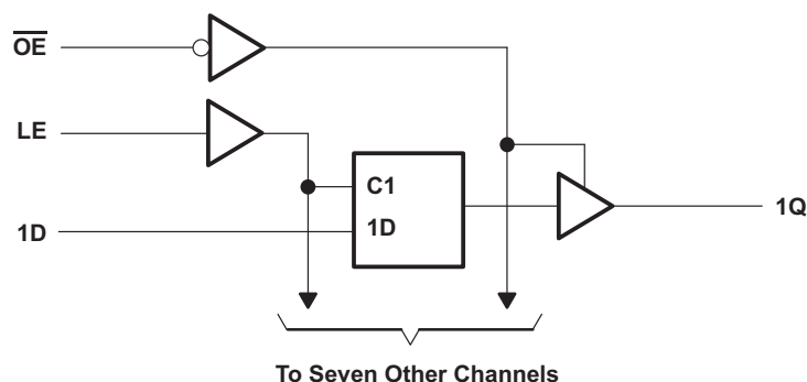
Simplified Schematic
